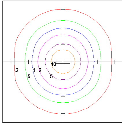
SOLAR ILLUMINATIONS 20W VAPOR LIGHT WITH CLEAR LENS. Horizontal Footcandles Scale: 1 Inch = 10 FT. Light Loss Factor = 1.00 Lumens Per Lamp = 2460 Total Lamp Lumens = 2460 Mounting Height = 10.00 FT
