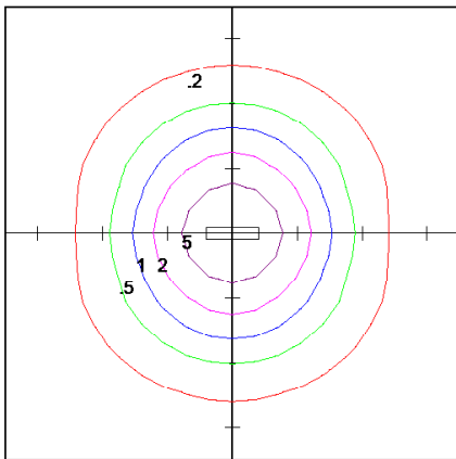
SOLAR ILLUMINATIONS 20W VAPOR LIGHT WITH CLEAR LENS. Horizontal Footcandles Scale: 1 Inch = 10 FT. Light Loss Factor = 1.00 Lumens Per Lamp = 1360 Total Lamp Lumens = 1360 Mounting Height = 10.00 FT
