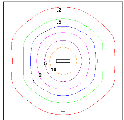
SOLAR ILLUMINATIONS 20W VAPOR LIGHT WITH CLEAR LENS. Horizontal Footcandles Scale: 1 Inch = 10 FT. Light Loss Factor = 1.00 Lumens Per Lamp = 2460 Total Lamp Lumens = 2460 Mounting Height = 10.00 FT
